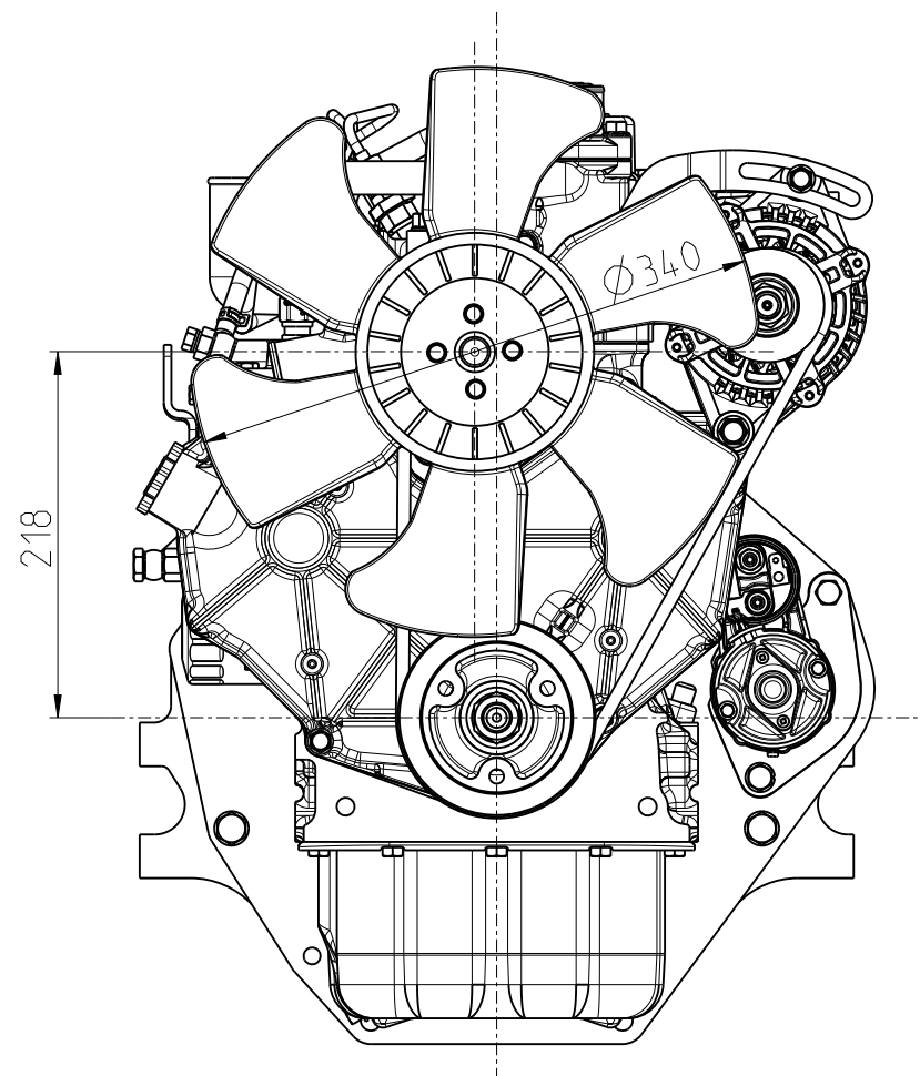
Constant-Speed (6 BLADE PUSHING-FAN)
