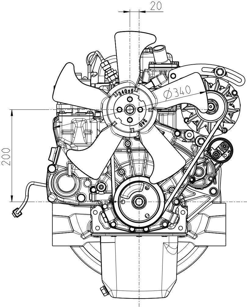
Variable-Speed (5 BLADE SUCTION-FAN)
