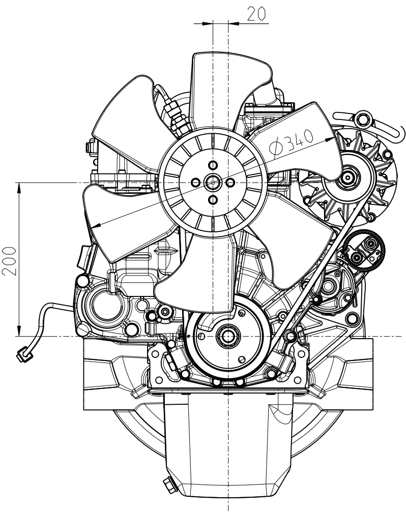
Constant-Speed (6 BLADE PUSHING-FAN)
