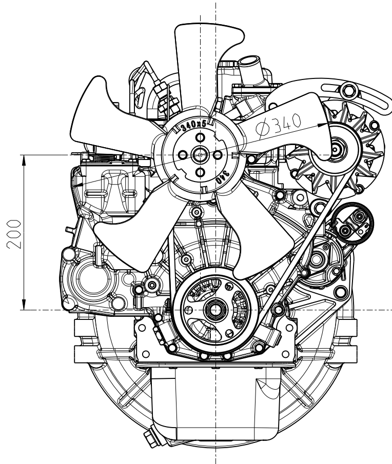
Variable-Speed (5 BLADE SUCTION-FAN)
