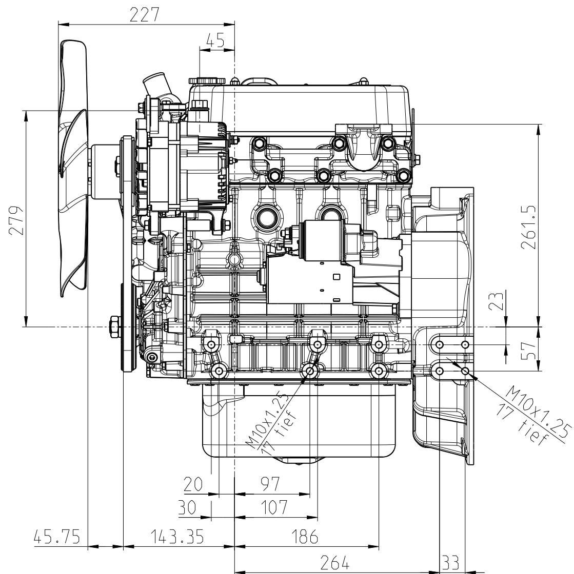
VS (5 BLADE SUCTION-FAN)
