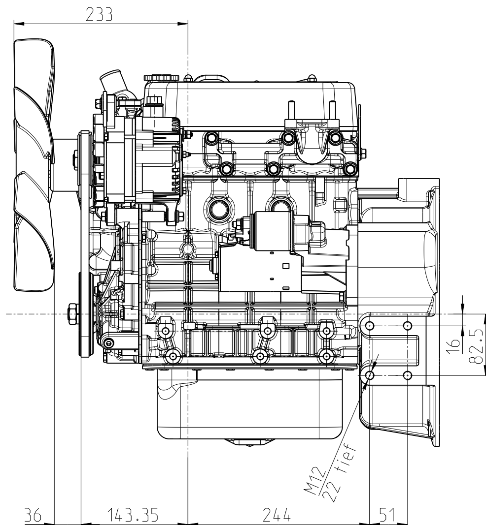
CS (6 BLADE PUSHING-FAN)
