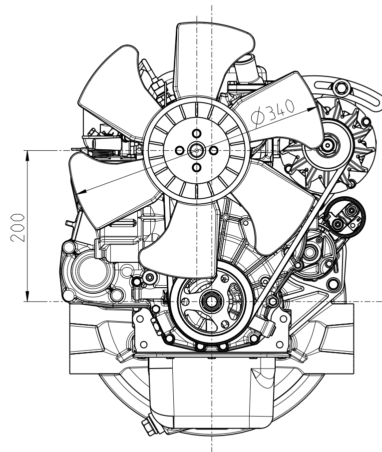
Constant-Speed (6 BLADE PUSHING-FAN)
